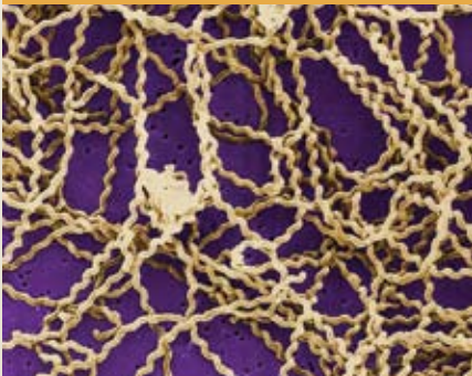
Scanned electron micrograph of Leptospira sp. bacteria (courtesy of Rob Weyant)
